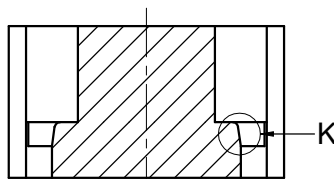
Section E-E
