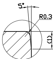
Detail G
