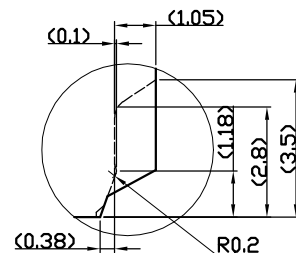
Detail Q
