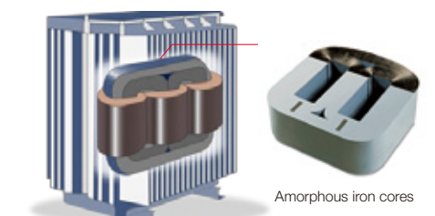
Transformer interior
